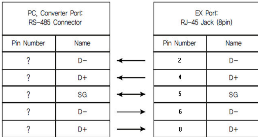
485 to 232 Converter
