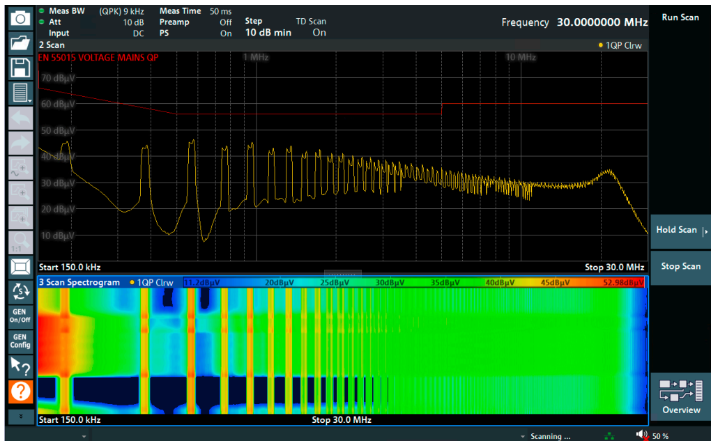
Analysis of the emissions of a LED lamp while changing the brightness levels. The measurement was made with a quasi-peak detector.
