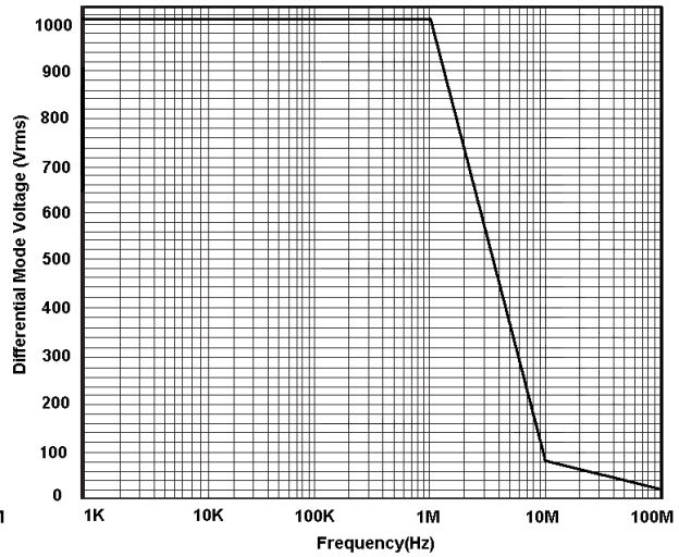
Figure 2: DP6150(A/B) Differential Mode Voltage VS Frequency
